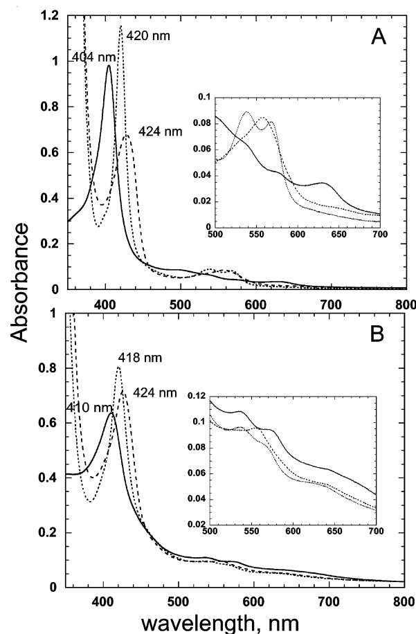
FIGURE 3: UV/visible absorption spectra of wild-type Hmx1 (A) and CaHmx1 (B) proteins. The spectra are of the ferric heme complex (—), the ferrous complex (— — —), and the ferrous carbon monoxide complex (- - -). The insets show an expanded region of the spectra.
