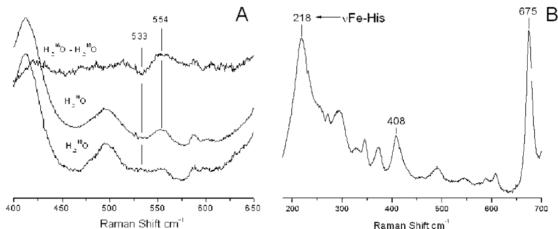
FIGURE 6: Low-frequency RR spectra of ferric Hmx1. (A) The RR spectra obtained in 25 mM CHES buffer (pH 9.5) in H 2 16 O and H 2 18 O with 413 nm excitation at room temperature. (B) The RR spectrum obtained with 442 nm excitation at room temperature.
